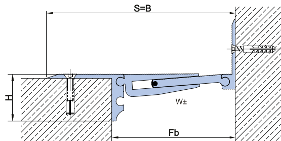
DEFLEX E 423/N-090
